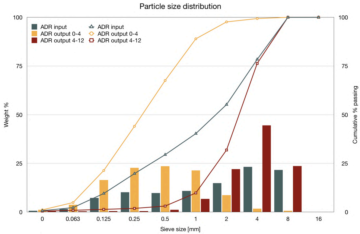
Figure B.1: Particle size distribution graph
