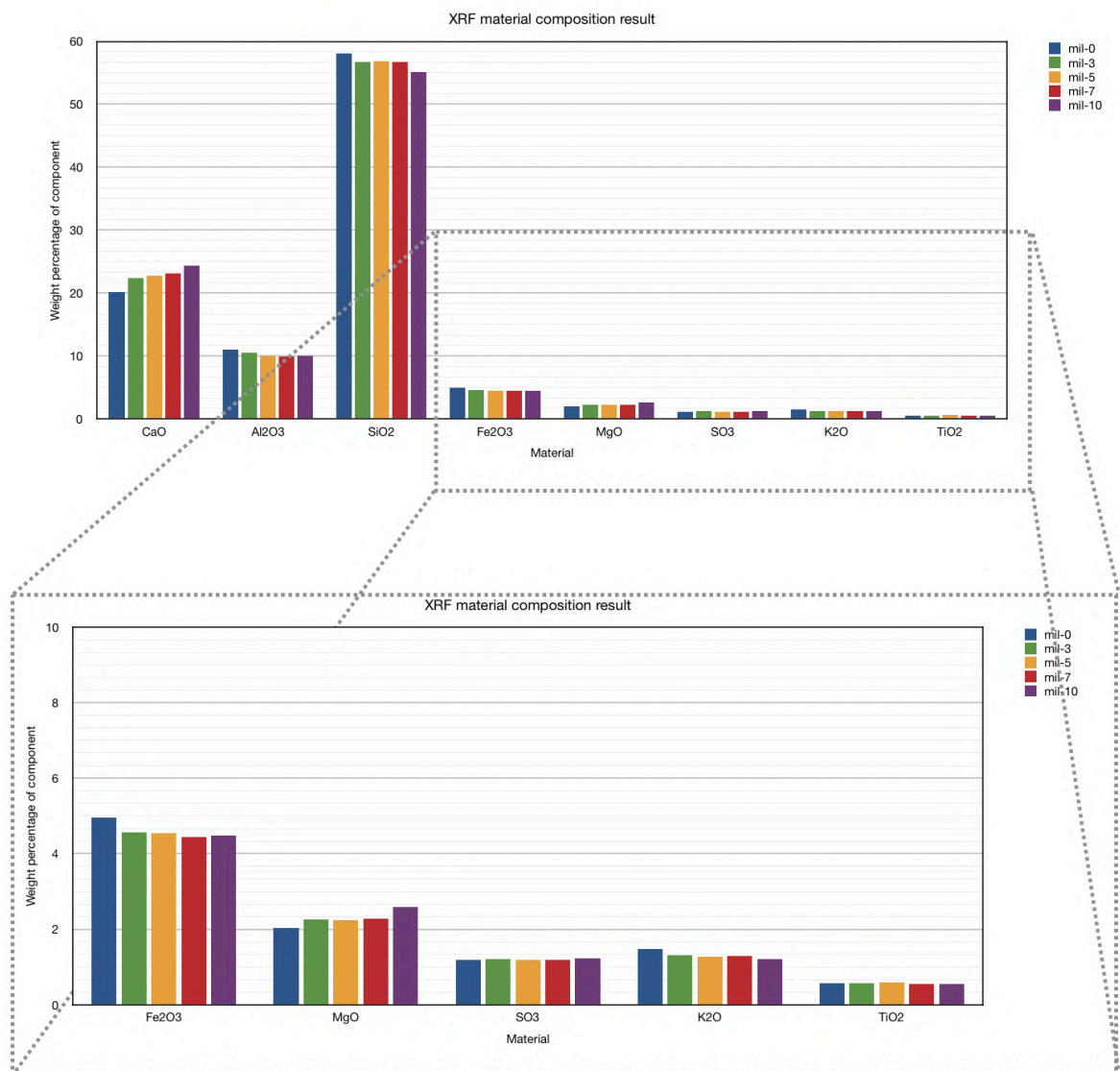
Figure 5.11: XRF results
