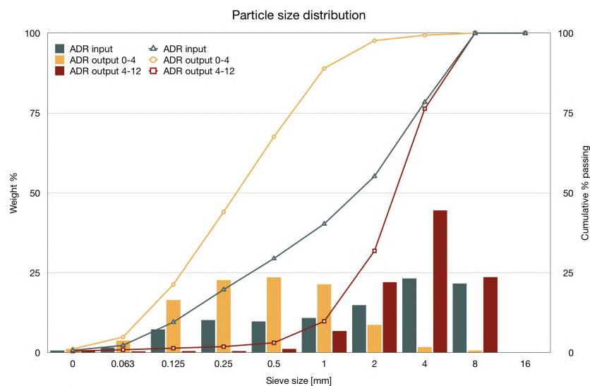
Figure 5.1: Particle size distribution
