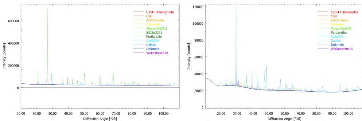
Figure F.6: Mil-10 XRD chart [3/3]
