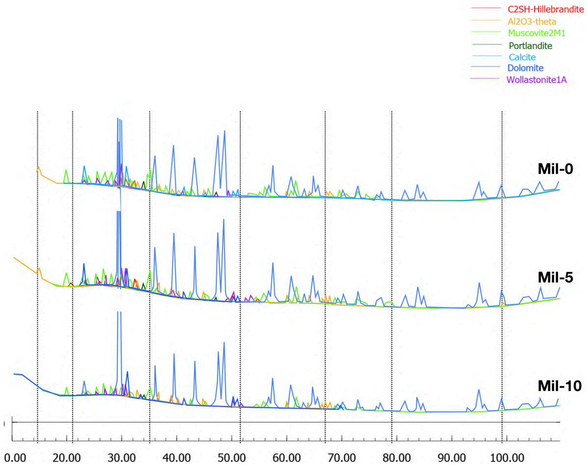
Figure 5.12: XRD graphical results
