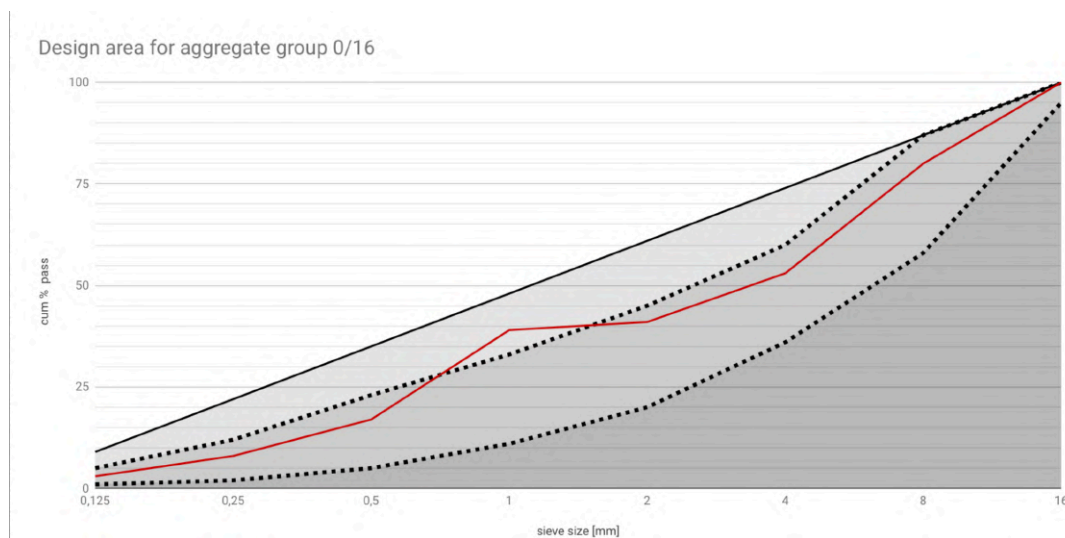
Figure 5.6: PSD for mix design
