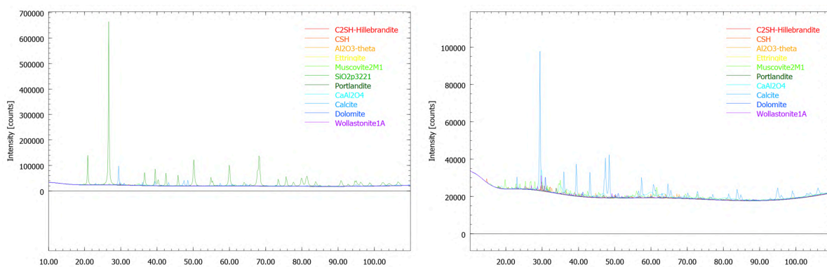
Figure F.4: Mil-0 XRD chart [1/3]
