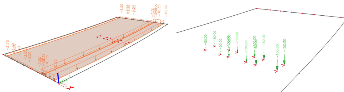
Figure 3.12: Traffic load (left: UDL and right: TS) applied to the orthotropic plate model (curved bridge deck)
