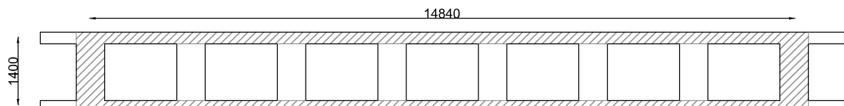
Figure 3.6: Area taken into account to calculate the torsional stiffness
