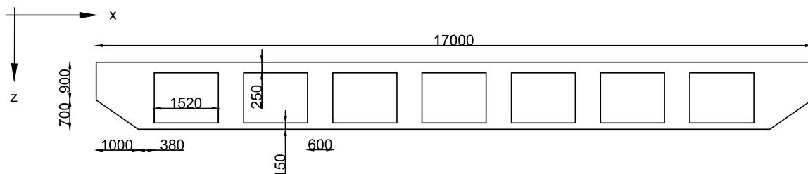
Figure 2.1: Cross-section of the bridge decks used for the Blankenburgverbinding (mm)
