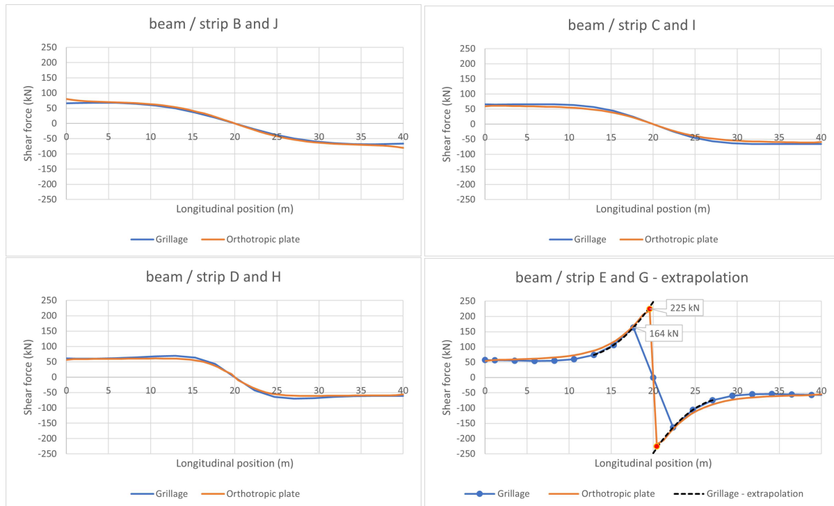
Figure 7.22: Shear forces LC7
