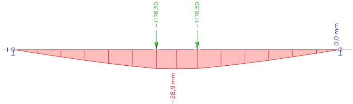
Figure 6.7: Deflection transverse strip grillage model ( w_{max} = 28.9 \text{ mm} )
