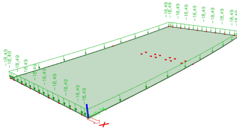
Figure 3.10: Self-weight applied to the orthotropic plate model
