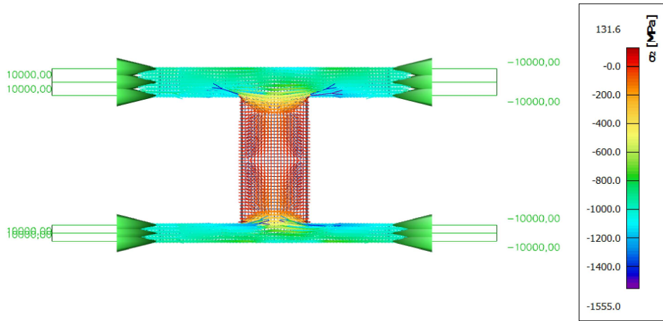
Figure 5.9: Trajectories major principle stress
