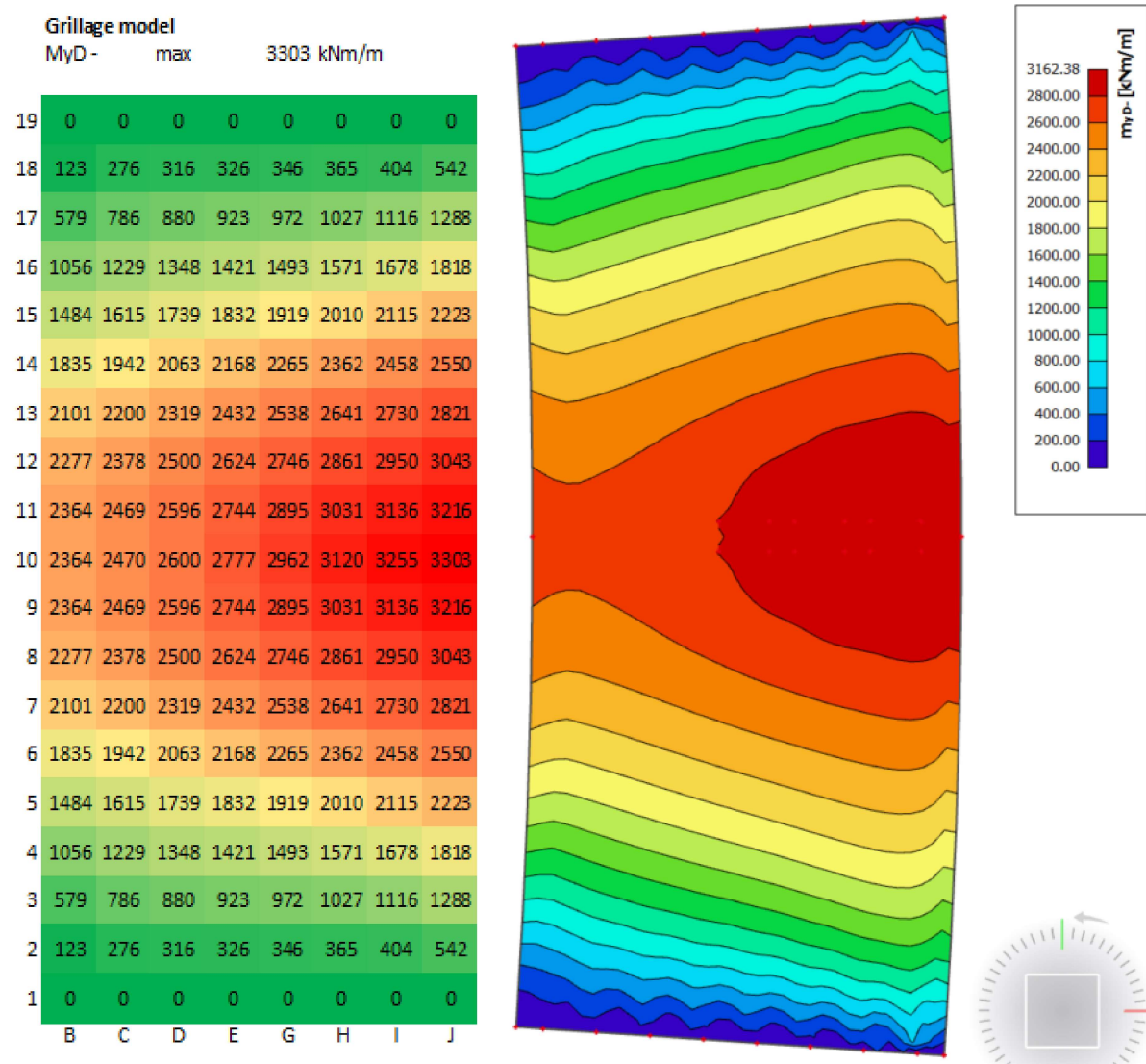
Figure 8.6: MyD-, grillage model (left) and orthotropic plate model (right) (kNm/m)
