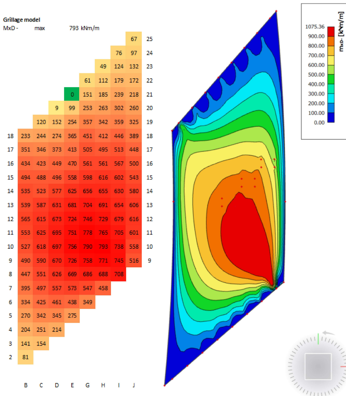
Figure G.2: MxD-, grillage model (left) and orthotropic plate model (right) (kNm/m)
