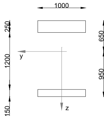
Figure 3.4: Cross-section for bending in x -direction (mm)
