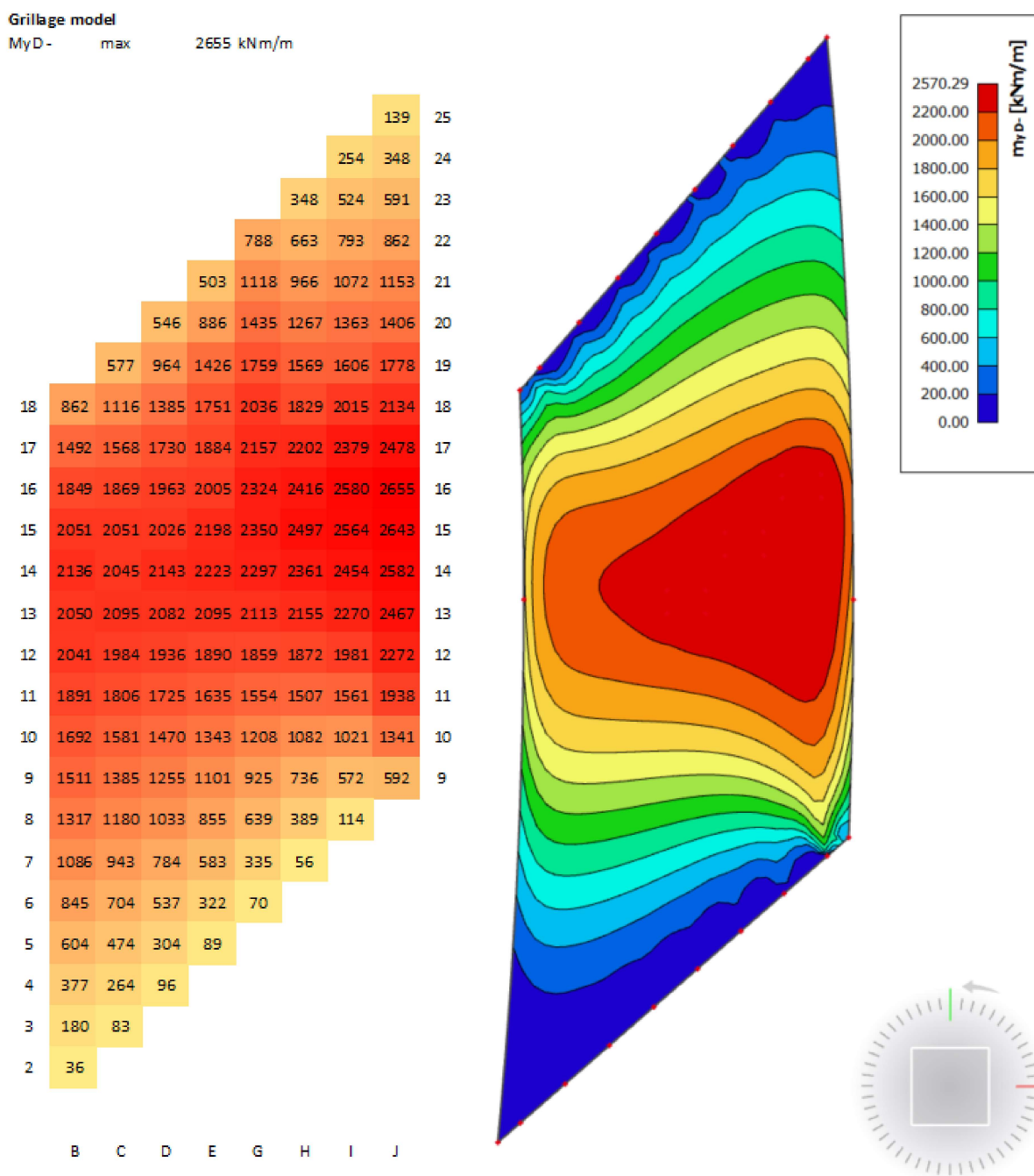
Figure G.4: MyD-, grillage model (left) and orthotropic plate model (right) (kNm/m)
