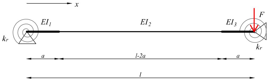
Figure C.6: Semi-rigid supported beam with support settlement
