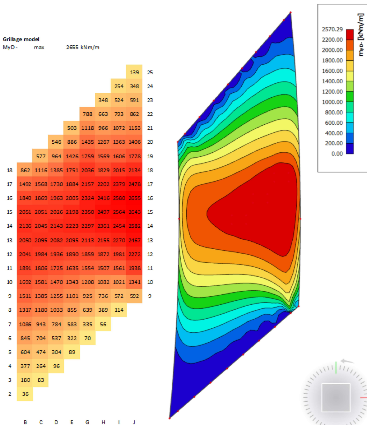
Figure 9.6: MyD-, grillage model (left) and orthotropic plate model (right) (kNm/m)
