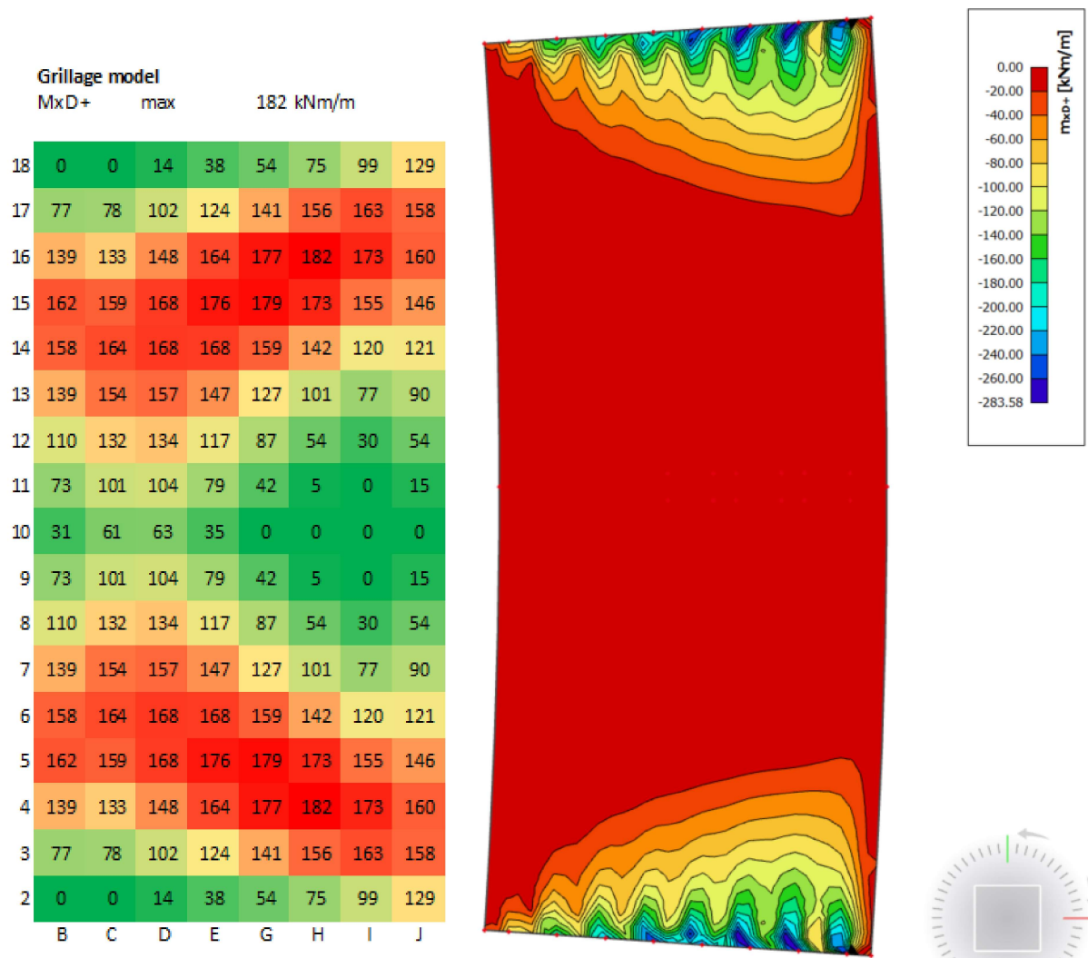
Figure F.1: MxD+, grillage model (left) and orthotropic plate model (right) (kNm/m)
