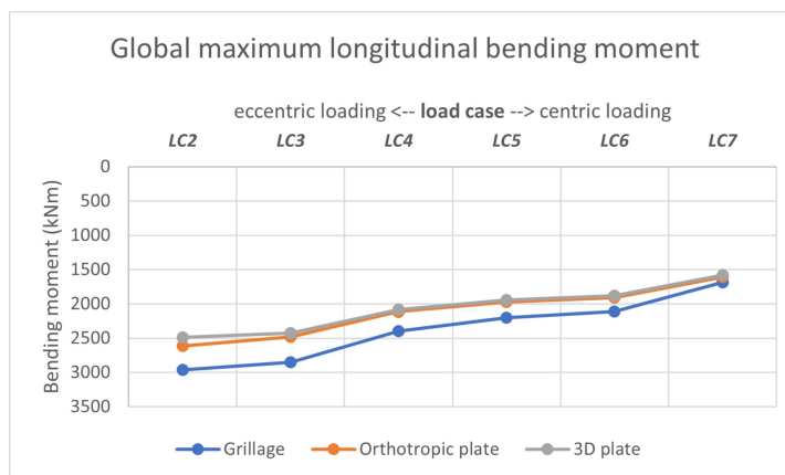
Figure 7.10: Global maximum longitudinal bending moment
