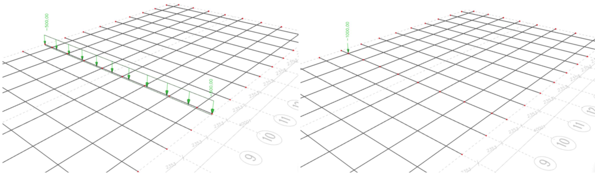
Figure 4.7: Grillage model loaded with LC1 (left) and LC3 (right)
