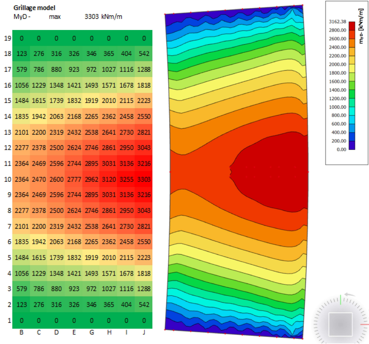
Figure F.4: MyD-, grillage model (left) and orthotropic plate model (right) (kNm/m)
