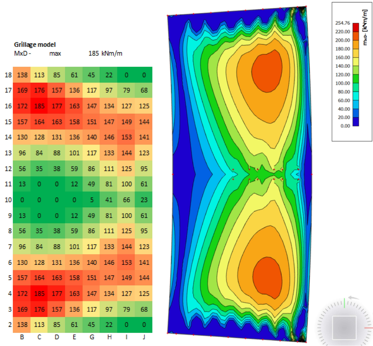
Figure F.2: MxD-, grillage model (left) and orthotropic plate model (right) (kNm/m)
