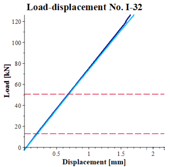
Figure 254: Load-displacement curves specimen I-32.
