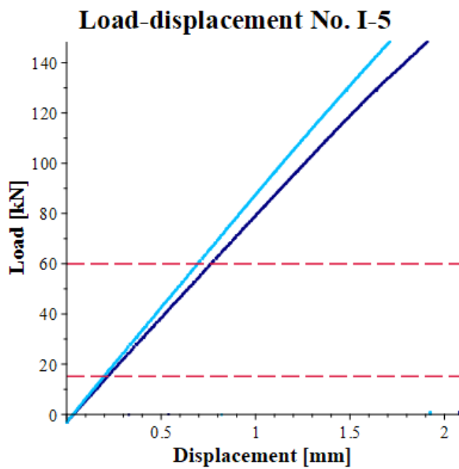
Figure 227: Load-displacement curves specimen I-5.
