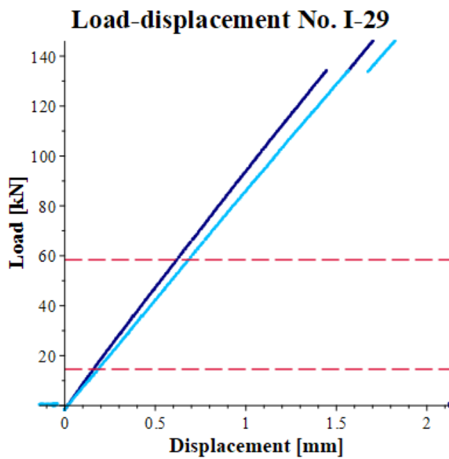
Figure 251: Load-displacement curves specimen I-29.
