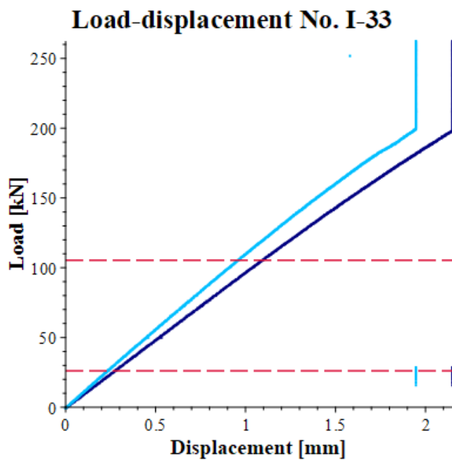
Figure 255: Load-displacement curves specimen I-33.
