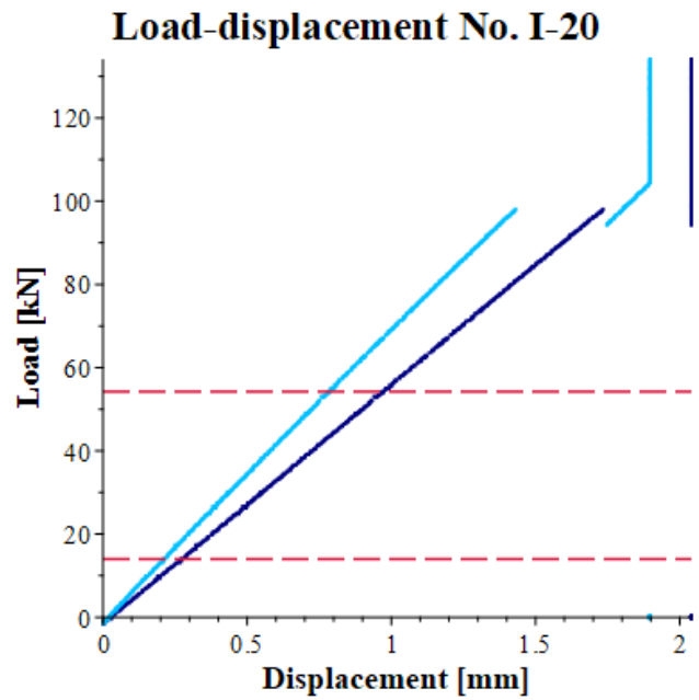
Figure 242: Load-displacement curves specimen I-20.
