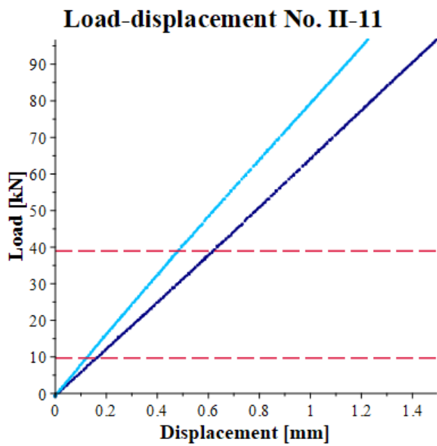
Figure 271: Load-displacement curves specimen II-11.
