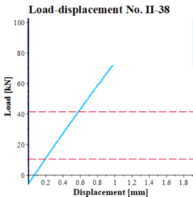
Figure 298: Load-displacement curve specimen II-38.
