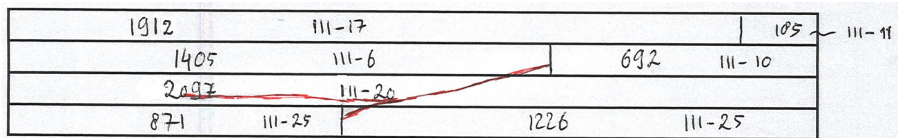
Figure 76: Beam layup and crack formation of specimen IV-3.
