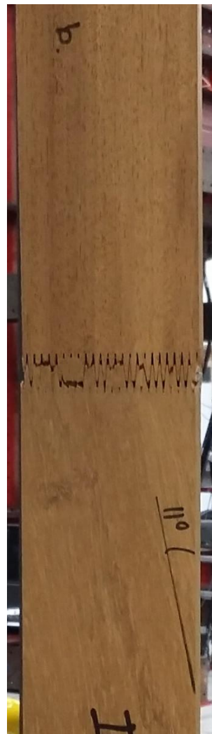
Figure 69: Failure of both fingers and glue (II-24).
