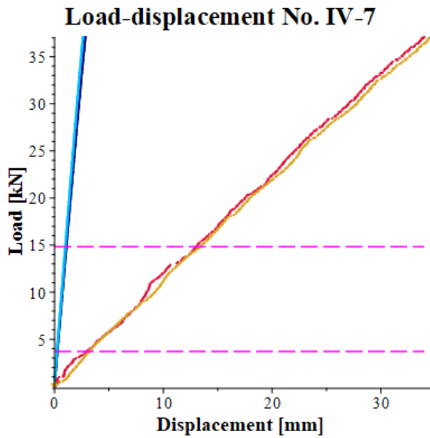
Figure 305: Load-displacement curves specimen IV-7.
