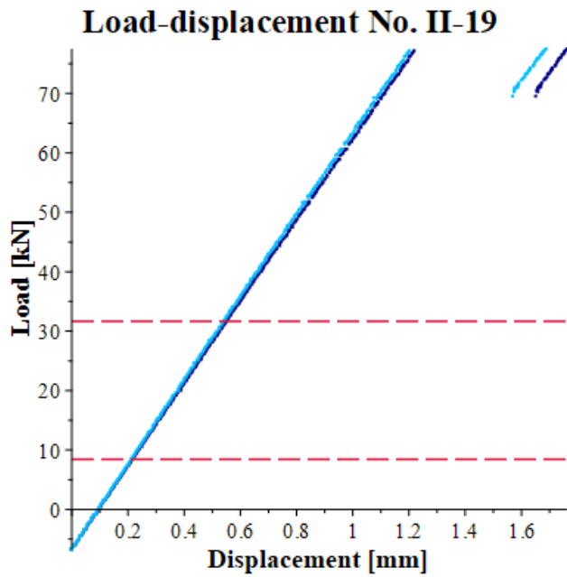
Figure 279: Load-displacement curves specimen II-19.
