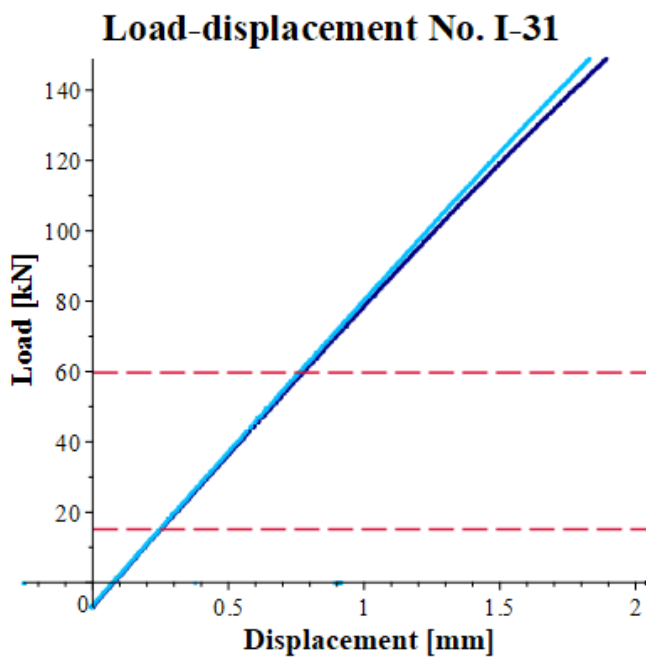
Figure 253: Load-displacement curves specimen I-31.
