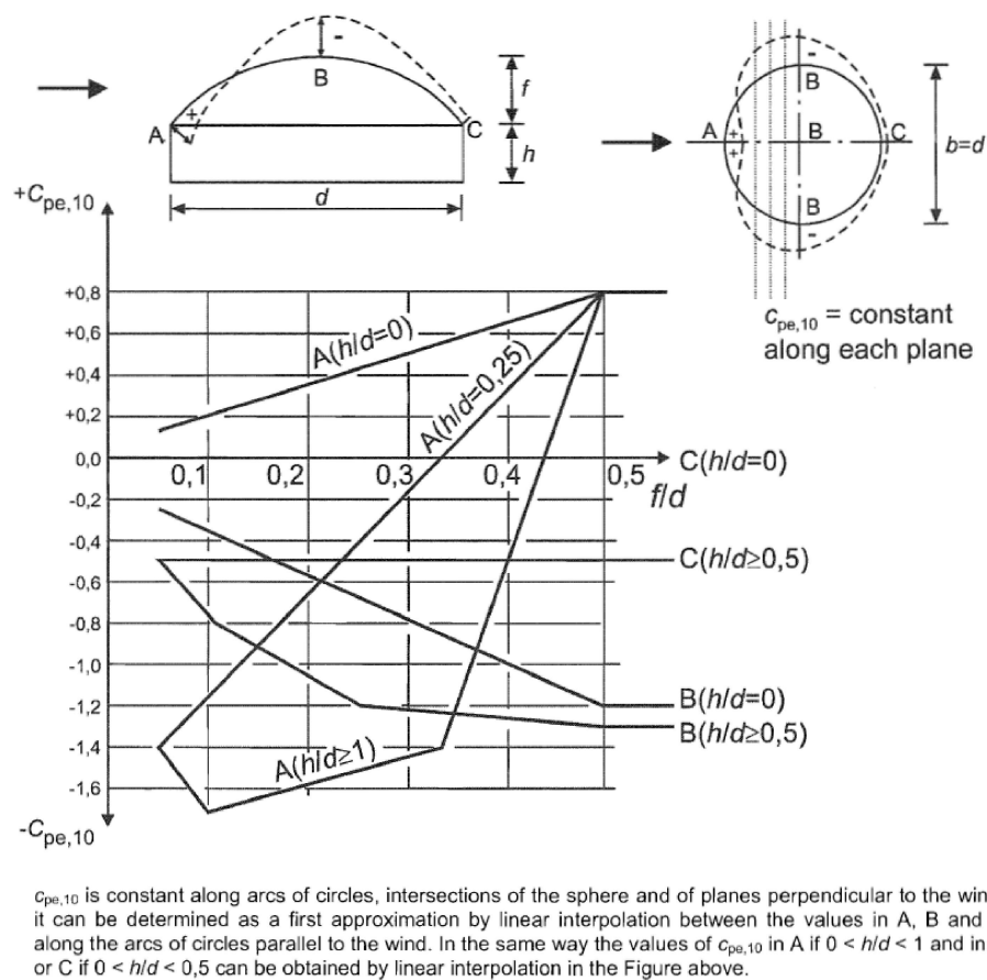
Figure 5.1: Pressure coefficient determination according to EN 1991-1-4, 7.2.8
