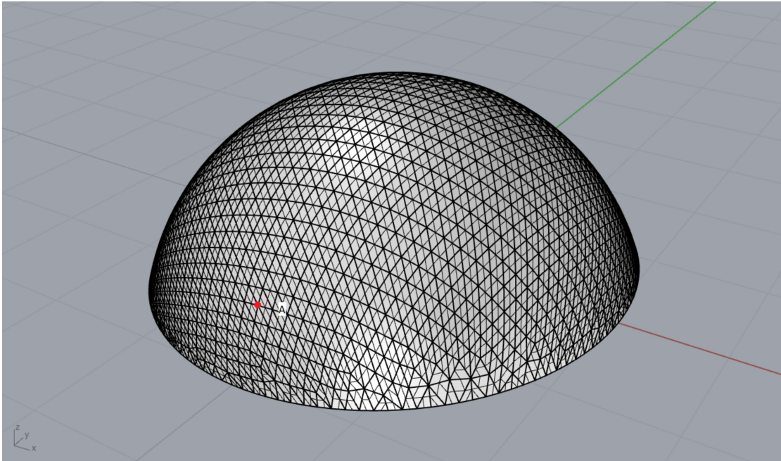
Figure 4.4: Model-2 maximum deformation point when subjected to undeformed loading case
