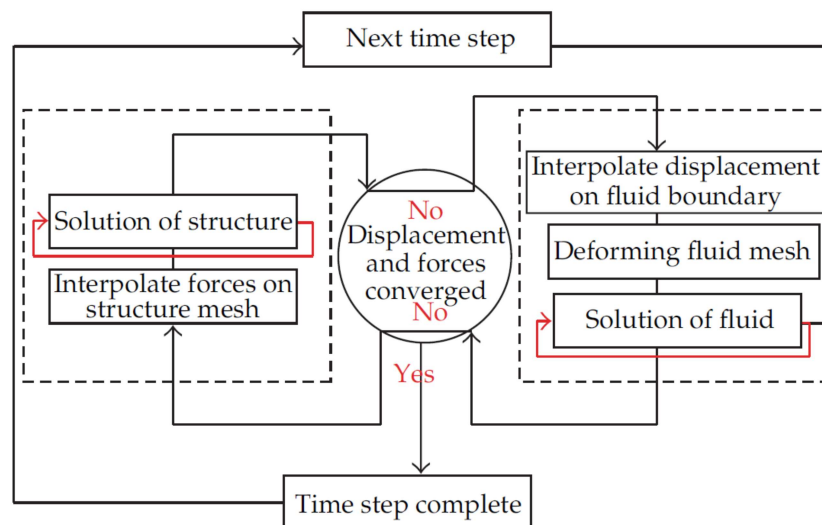
Figure 4.2: Two-way coupling
