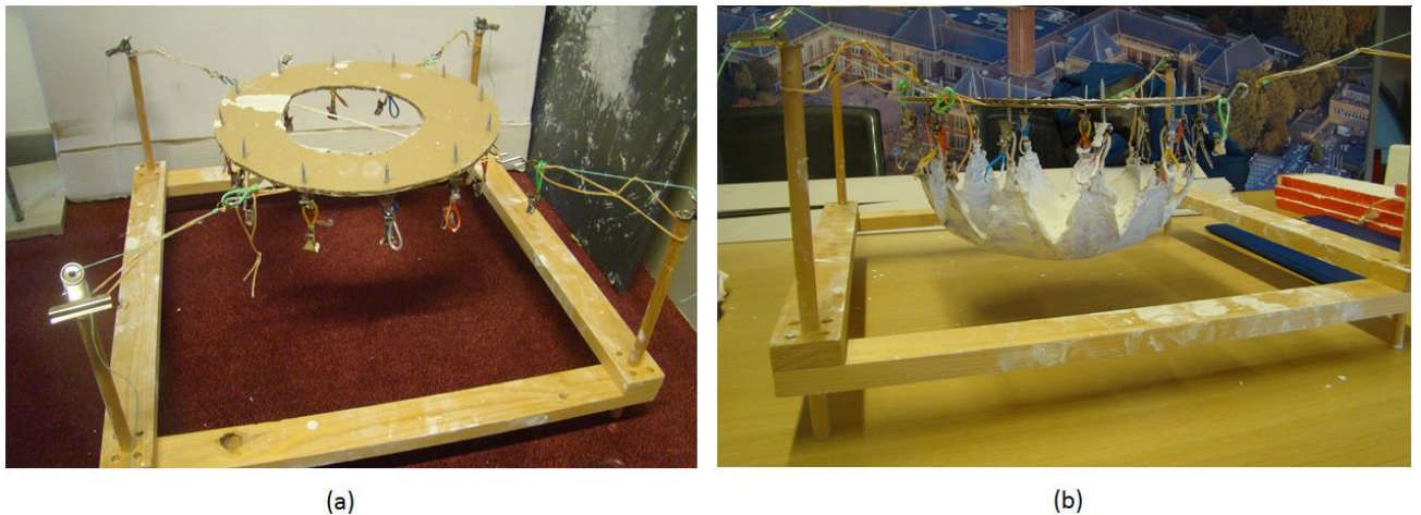
Figure 5-4: Supporting framework for the hanging model
