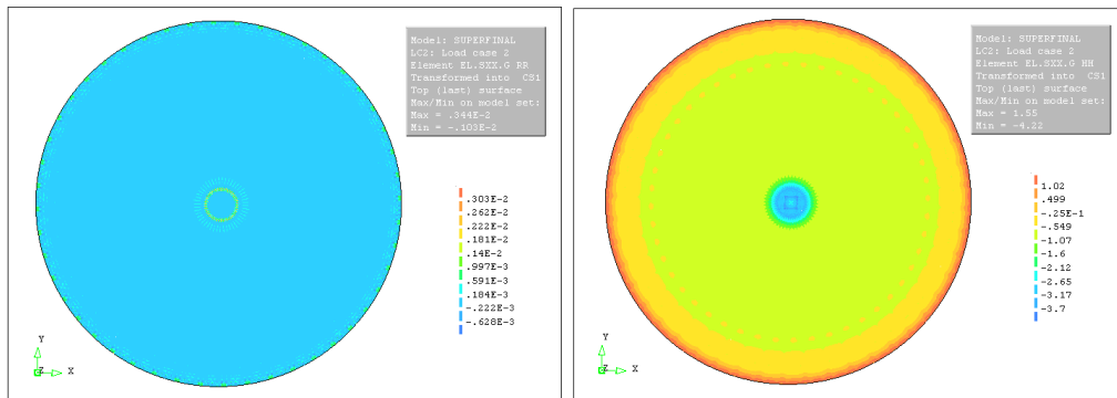
Figure D-1: Ring and Hoop stresses on the top surface of the shell for LC2
