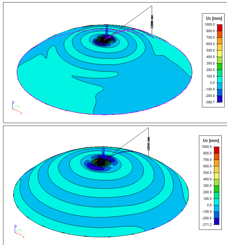
Figure 10-2: Design 1: First buckling mode for t=150 and 200 mm, for load combination 1
