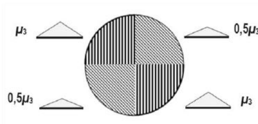
Figure 9-5: Snow load shape coefficients for dome [10]
