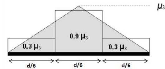
Figure 9-6: Loading scheme for redistributed snow [10]
