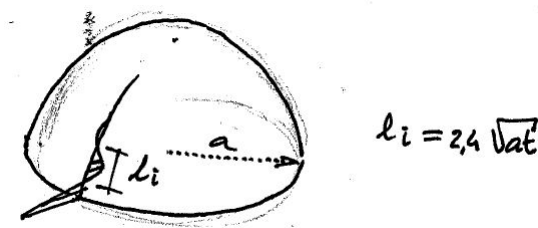
Figure 2-6: Influence length of edge in for a spherical dome [1]
