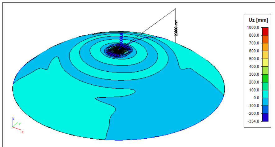
Figure 10-1: Design 1: First buckling mode for t=100 load combination 1
