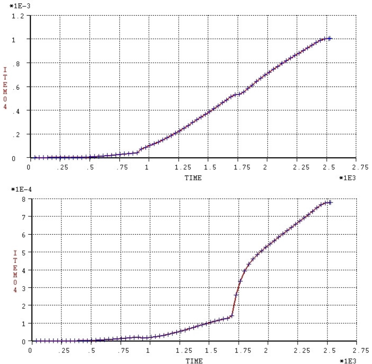
Two crack width-time relationships for two adjacent elements in the crack in the roof adjacent to the middle wall.
