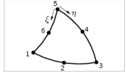
A CT12M element. Image taken from the DIANA manual (TNO DIANA, 2007)
