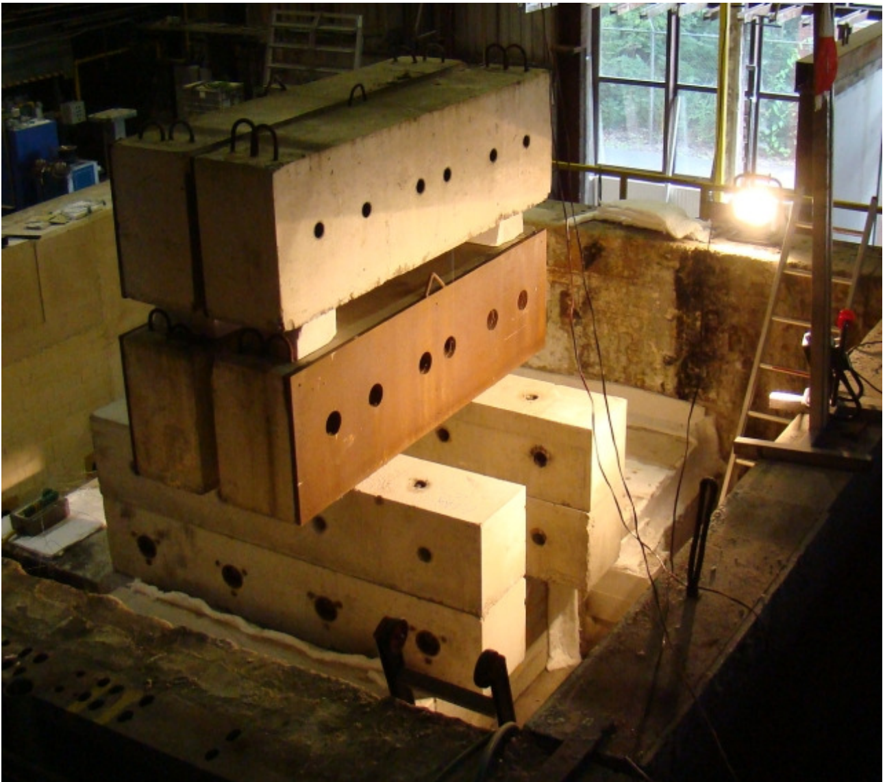
The construction of blocks used to put load on the specimen. The specimen itself is somewhere below all this.
