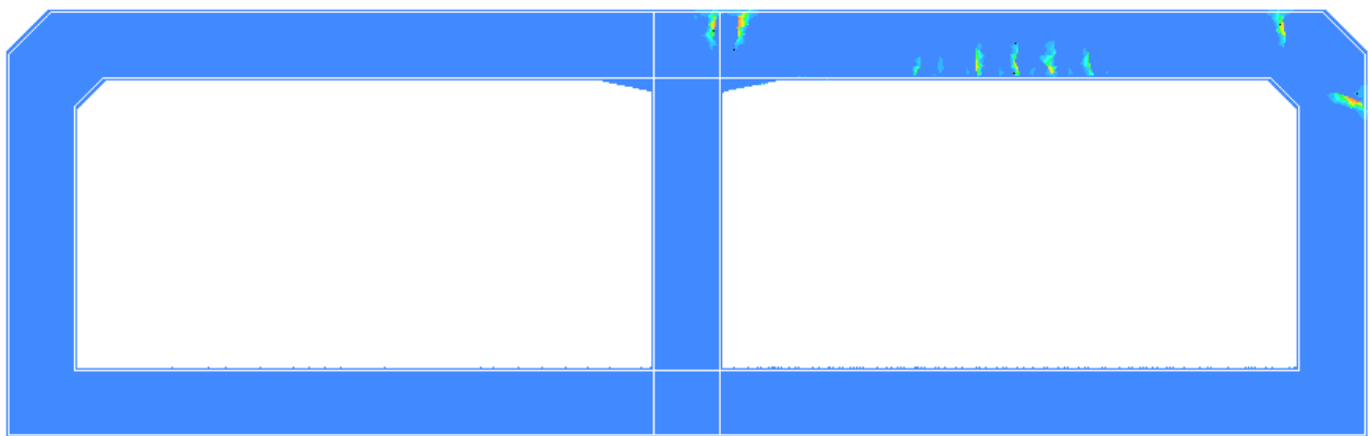
A plot of the fictitious crack width w clearly showing two parallel cracks in the roof adjacent to the middle wall. This plot has been obtained for a compressive strength reduced to 15 N/mm 2 .
