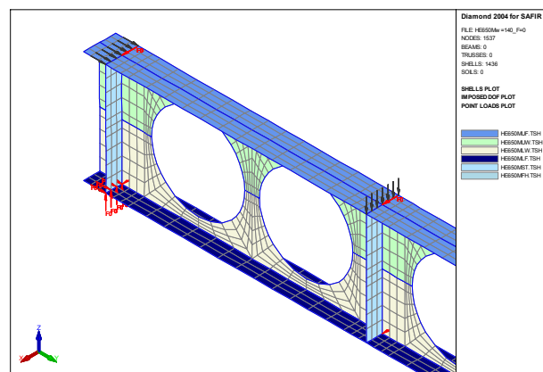
Figure 9.22 HE650M with s_0 = 140 mm
