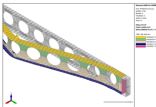
Figure 7.6 Deformation plot in Diamond
