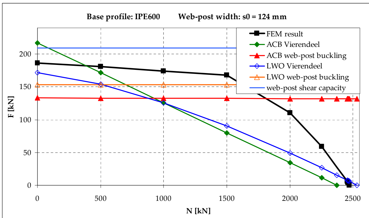
Figure 9.16 Results for web-post buckling parameter study: IPE600 with s_0 = 124 mm
