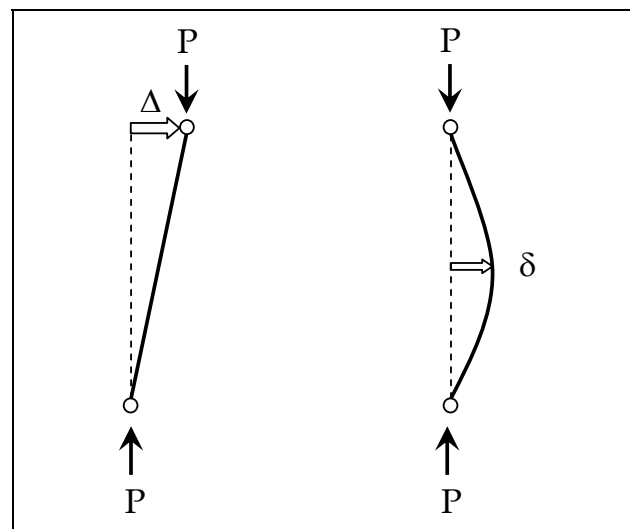
Figure 5.1 P - \Delta : sway displacement P - \delta : initial bow displacement
