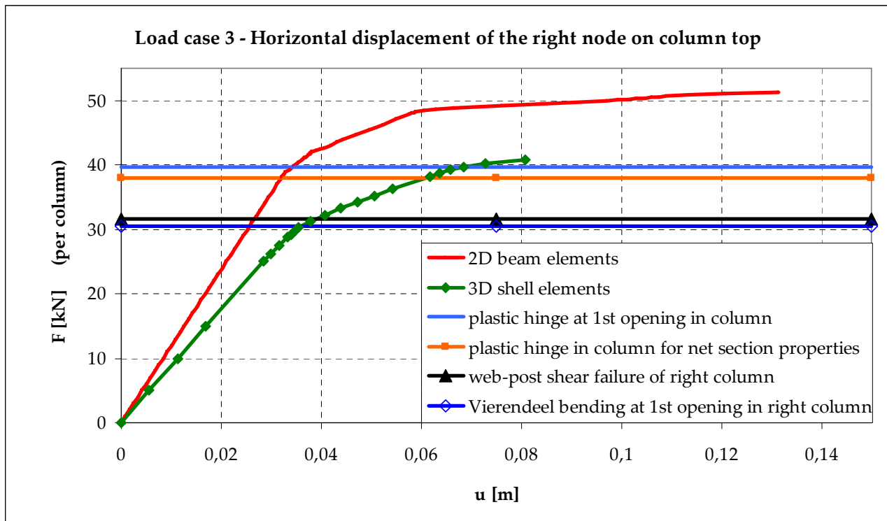
Figure 10.13 Load case 3: Load-displacement graphs for horizontal displacement of right node on column top
