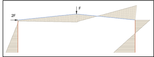
Figure 10.12 LC 3: combination of both vertical and horizontal point load
