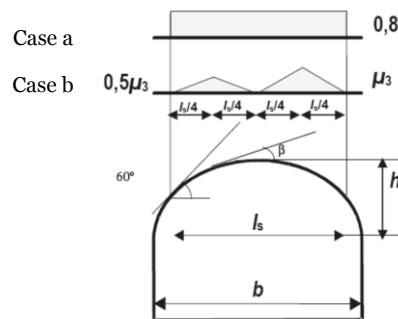
Fig.D7. Snow load shape coefficients for cylindrical roofs [3]
