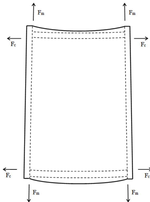
Fig. D52. Tensile forces on local connections
