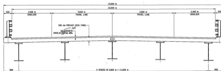
Fig.Ap3.30. Transverse bridge section of precast panels and centerline UHPPC joint fill
