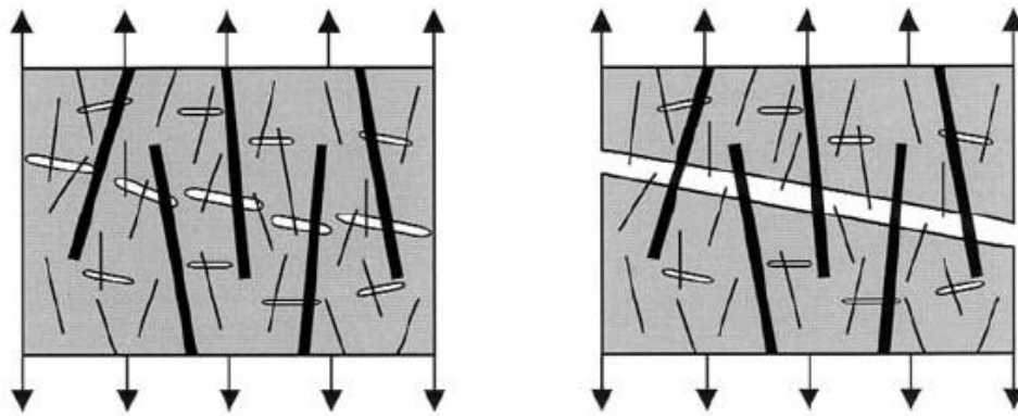
Fig. A3. Left: Activating of short fibers by micro cracking Right: Activating of long fibers by macro cracking [35]
