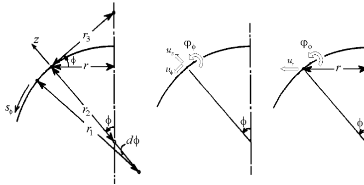
Fig.B9. Geometry of the meridian and positive directions of the displacements
