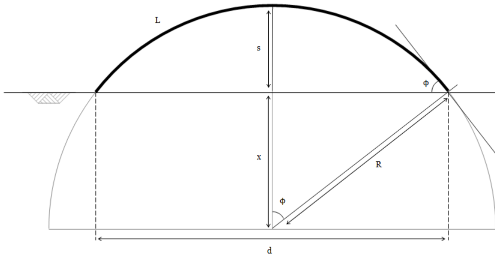
Fig.B26. Proportions in shell design
