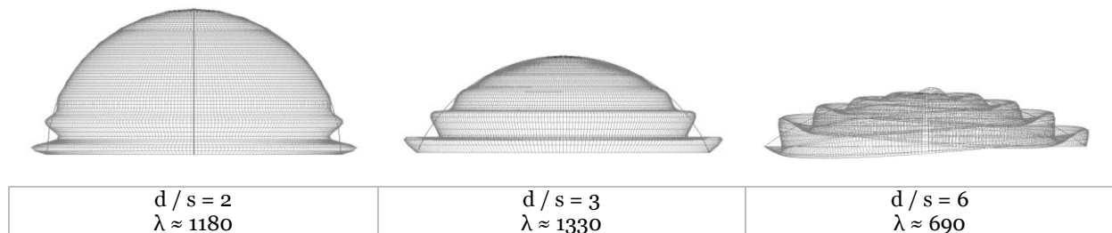
Fig.D33b. Buckling figures for shells subjected to vertical load t = 400mm
