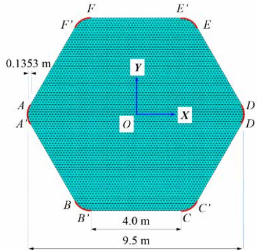
FIGURE 8.12 Initial conditions of Model B (shell with outward-curved supports).
