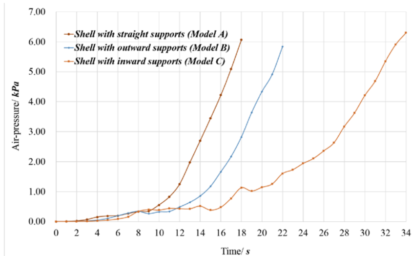
FIGURE 9.10 Changes in the air-pressure during tests of the three shell models.
