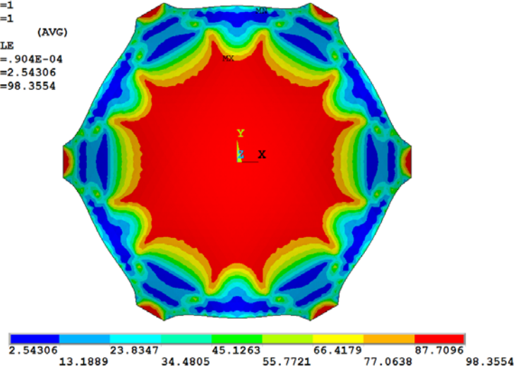
FIGURE 6.5 Stress ratio R_1 of Example 6.1 under self-weight (%).
