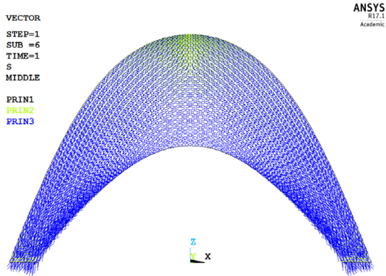
FIGURE 8.33 Vectorial representation of the principal stresses for Model A s (shell with simply supported straight supports) when the shell fails (lateral view).
