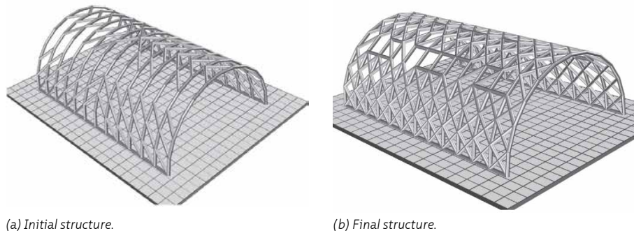
FIGURE 3.15 Example of discrete structure [90].
