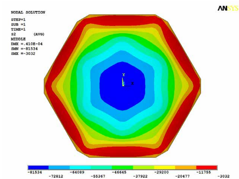
FIGURE 5.52 Principal stress S_2 at the middle surface of the shell of Example 5.4 (Pa).
