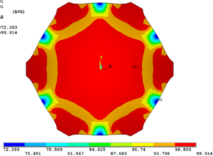
FIGURE 5.29 Stress ratio R_2 of Example 5.2 under loads with a same distribution as the hanging membrane (%).
