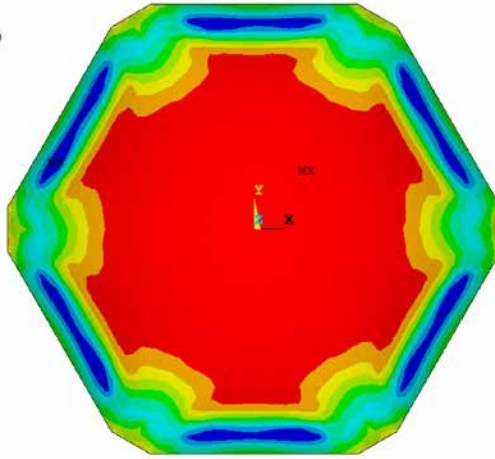
FIGURE 5.56 Stress ratio R_1 of Example 5.4 (%).
