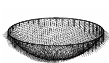
(a) Integral cable-net structure of FAST [73].
