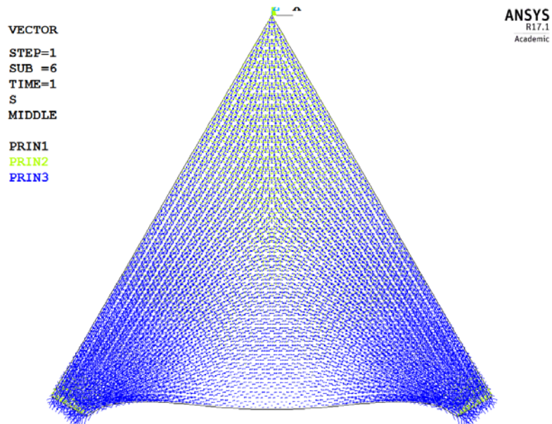
FIGURE 8.32 Vectorial representation of the principal stresses for Model A_5 (shell with simply supported straight supports) when the shell fails.
