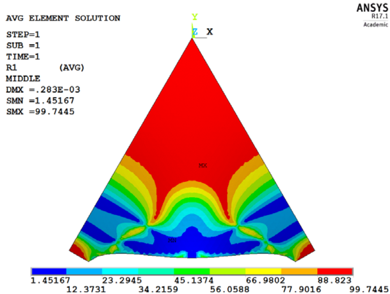
FIGURE 8.22 R_1 of Model A_5 (shell with simply supported straight supports; %).
