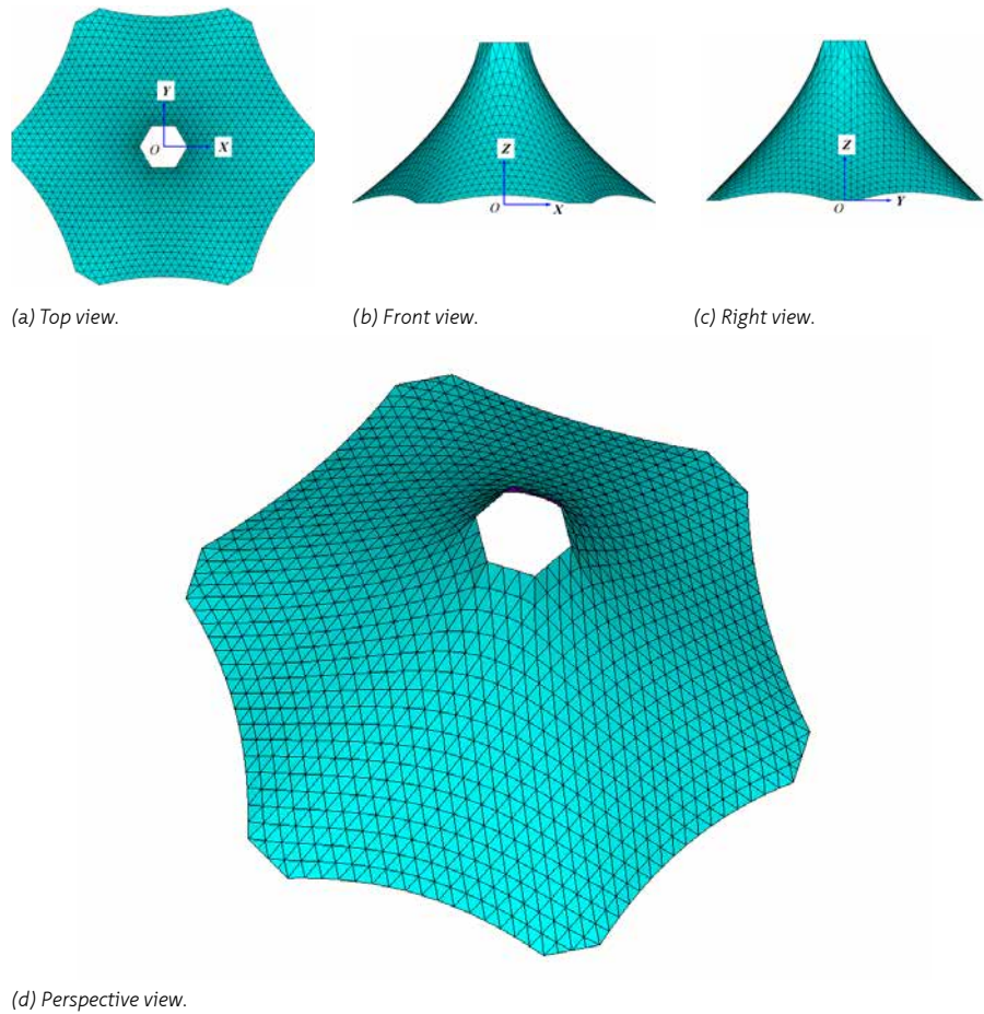
FIGURE 5.33 Form-Finding result of Example 5.3 .
