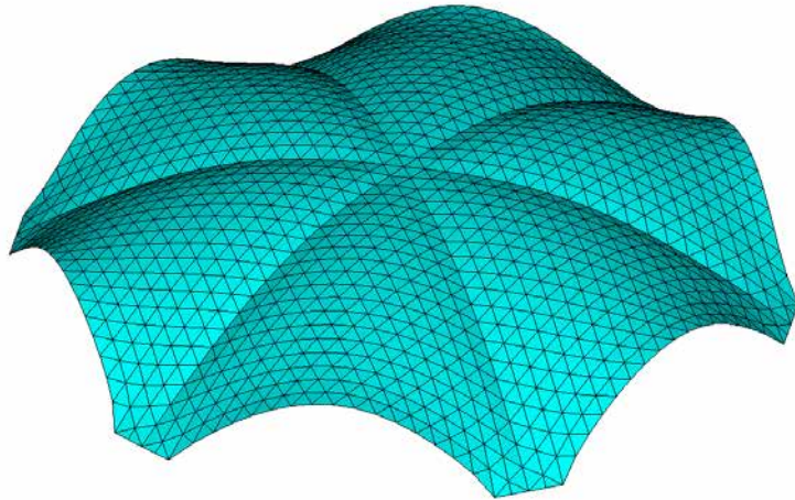
FIGURE 7.5 Four initial structural systems and Form-Finding results Example 7.4 .
