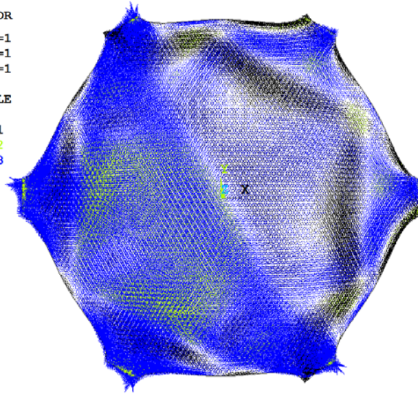
FIGURE 8.37 Vectorial representation of the principal stresses for Model A 6 (shell with simply supported straight supports) under half-span loads.
