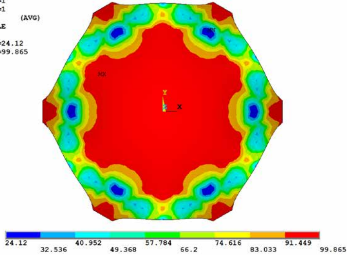
FIGURE 5.28 Stress ratio R_1 of Example 5.2 under loads with a same distribution as the hanging membrane (%).
