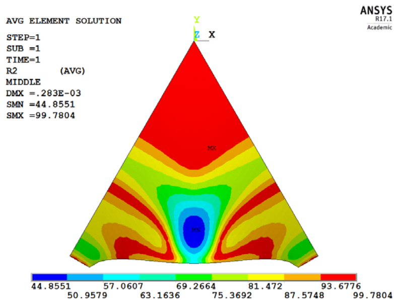
FIGURE 8.23 R_2 of Model A_5 (shell with simply supported straight supports; %).
