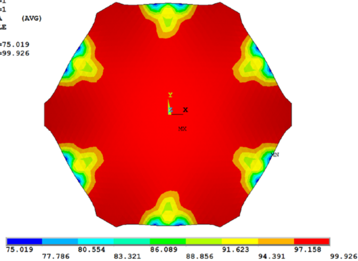
FIGURE 5.27 Strain-energy ratio \alpha of Example 5.2 (%).
