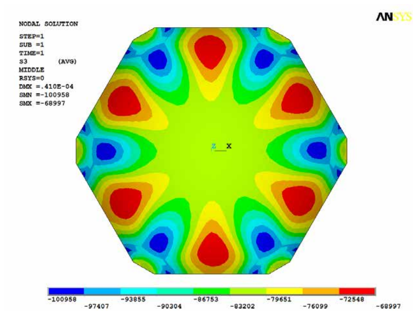
FIGURE 5.53 Principal stress S_3 at the middle surface of the shell of Example 5.4 (Pa).
