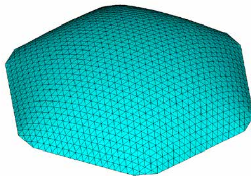
FIGURE 5.47 Form-Finding result of Example 5.4 .
