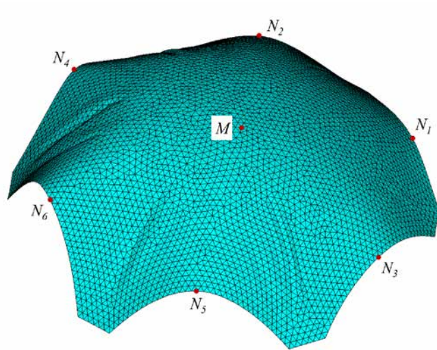
FIGURE 6.14 Form-Control result of Example 6.3 with a finer mesh.
