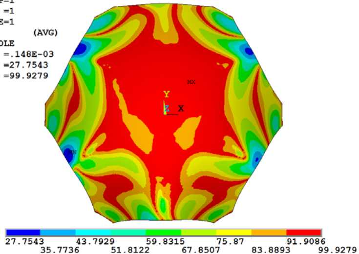
FIGURE 6.17 Stress ratio R_2 of Example 6.3 (%).
