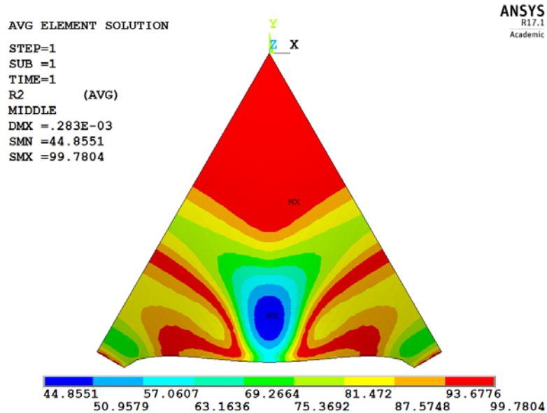
FIGURE 8.31 R_2 of Model A_5 (shell with simply supported straight supports) when the shell fails (%).
