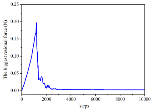
FIGURE 5.8 Evolution curve of the VFIFE method of Example 5.1 .
