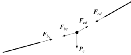
FIGURE 5.5 Residual force of particle c.
