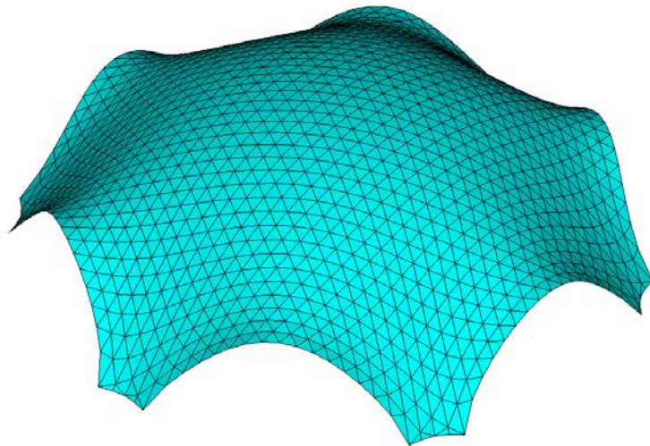
(c) Initial conditions of Example 5.2 with inward-curved supports and the Form-Finding result.
