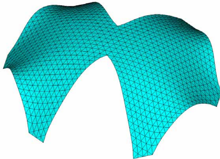
FIGURE 7.2 Two initial structural systems and Form-Finding results of Example 7.1.
