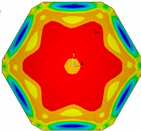
FIGURE 5.57 Stress ratio R_2 of Example 5.4 (%).
