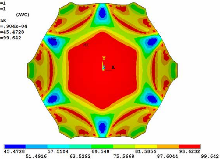
FIGURE 6.6 Stress ratio R_2 of Example 6.1 under self-weight (%).
