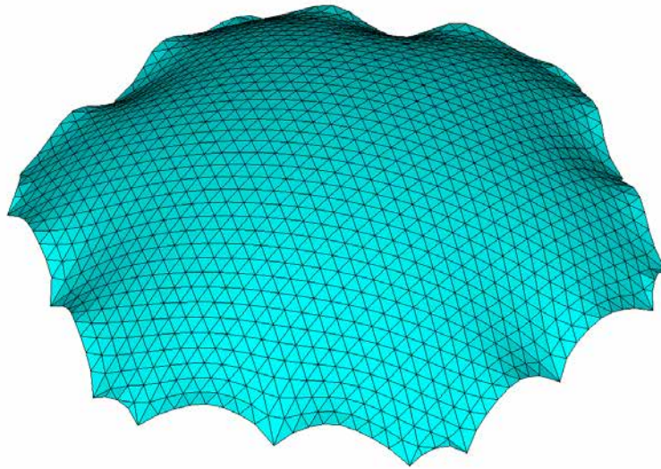
(b) Initial conditions of Example 5.2 with more point supports and the Form-Finding result.
