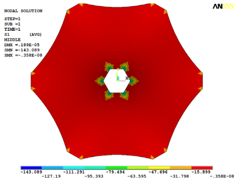
FIGURE 5.37 Principal stress S_1 at the middle surface of the shell of Example 5.3 (Pa).
