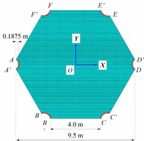
FIGURE 8.14 Initial conditions of Model D (shell with strongly inward-curved supports).
