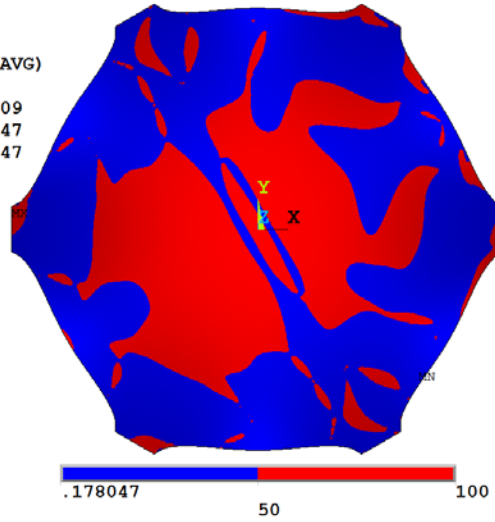
FIGURE 8.35 R_1 of Model A_5 (shell with simply supported straight supports) under half-span loads.
